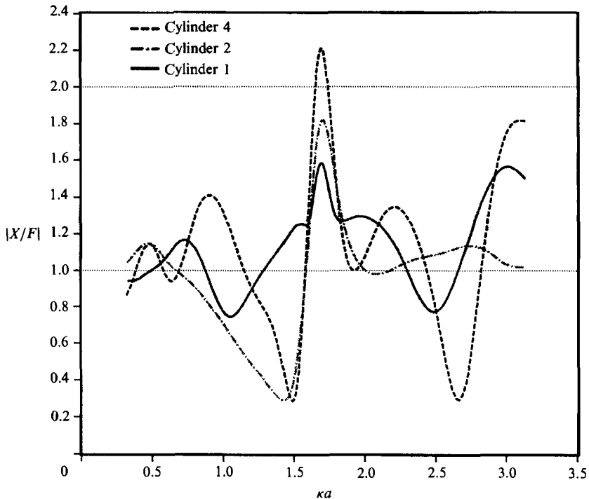
FIGURE C1. Non-dimensional amplitude of the first-order force in the direction of wave advance plotted against \kappa a for a group of four cylinders situated at the vertices of a square ( a/h = \frac{1}{2} , R/h = 2 , \beta = \frac{1}{4}\pi ).
